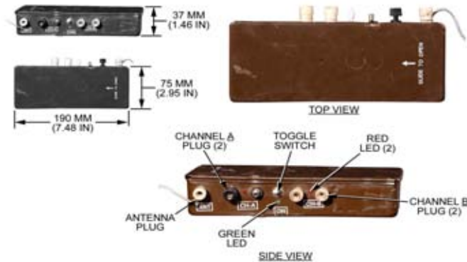
TERRORIST/INSURGENT & GUERRILLA ORG IMPROVED DEVICE, RADIO CONTROLLED (R/C), DTMF, BROWN BOX, MODEL UNKNOWN
