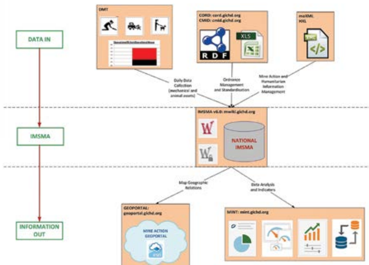
Figure 1. IMSMA Architecture. All graphics courtesy of GICHD.
